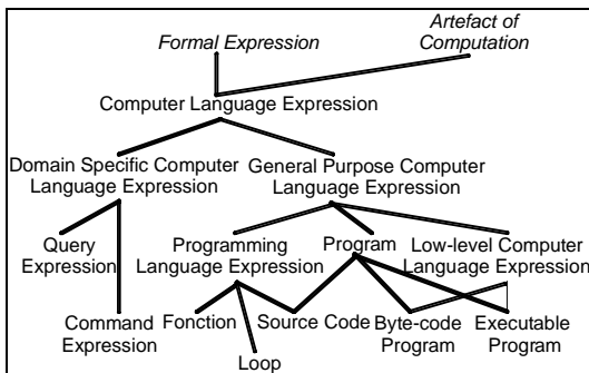
Figure 8: A sub-ontology of Programs in COPS.
