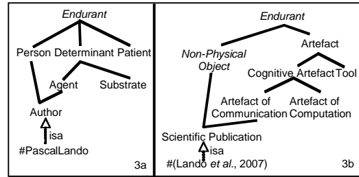
Figure 3: Modeling of roles (a) and functions-artefacts (b).
