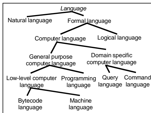
Figure 7: The sub-ontology of computer languages in COPS.
