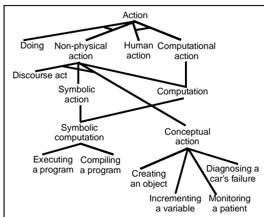
Figure 6: The sub-ontology of Actions in COPS
